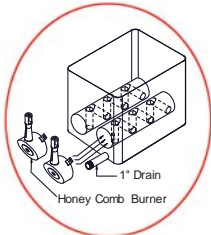
Tube-Fire Heating System for GDF12 & GDF11D
