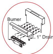
Tube-Fire Heating System
